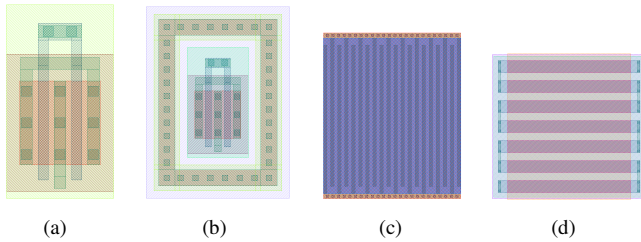
Fig. 2. Examples of generated devices from MAGICAL. (a) NMOS, (b) PMOS with guard ring, (c) MOM capacitor, and (d) poly resistor.
