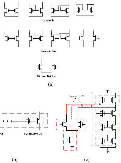
Fig. 3. Layout constraint extraction illustration. (a) Pattern library, (b) bias circuit symmetry detection, and (c) signal flow based traversal.
