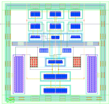
Fig. 6. Feed-forward compensated OTA circuit schematic, manual layout, and layout result from MAGICAL.
